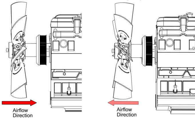
Blades Mounted for Sucker Fan (Pull)
